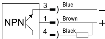
Fig. 7, NPN output type wiring
