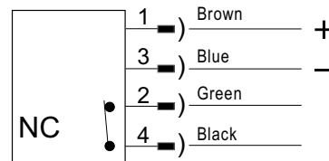
Fig. 11, Relay output type wiring (NC)
