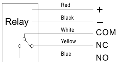
Fig. 9, Relay output type wiring
