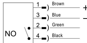
Fig. 10, Relay output type wiring (NO)
