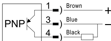
Fig. 8, PNP output type wiring
