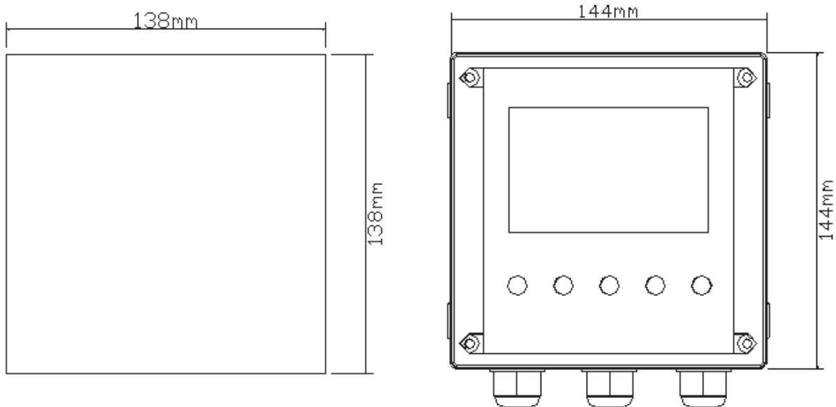
cutout size
