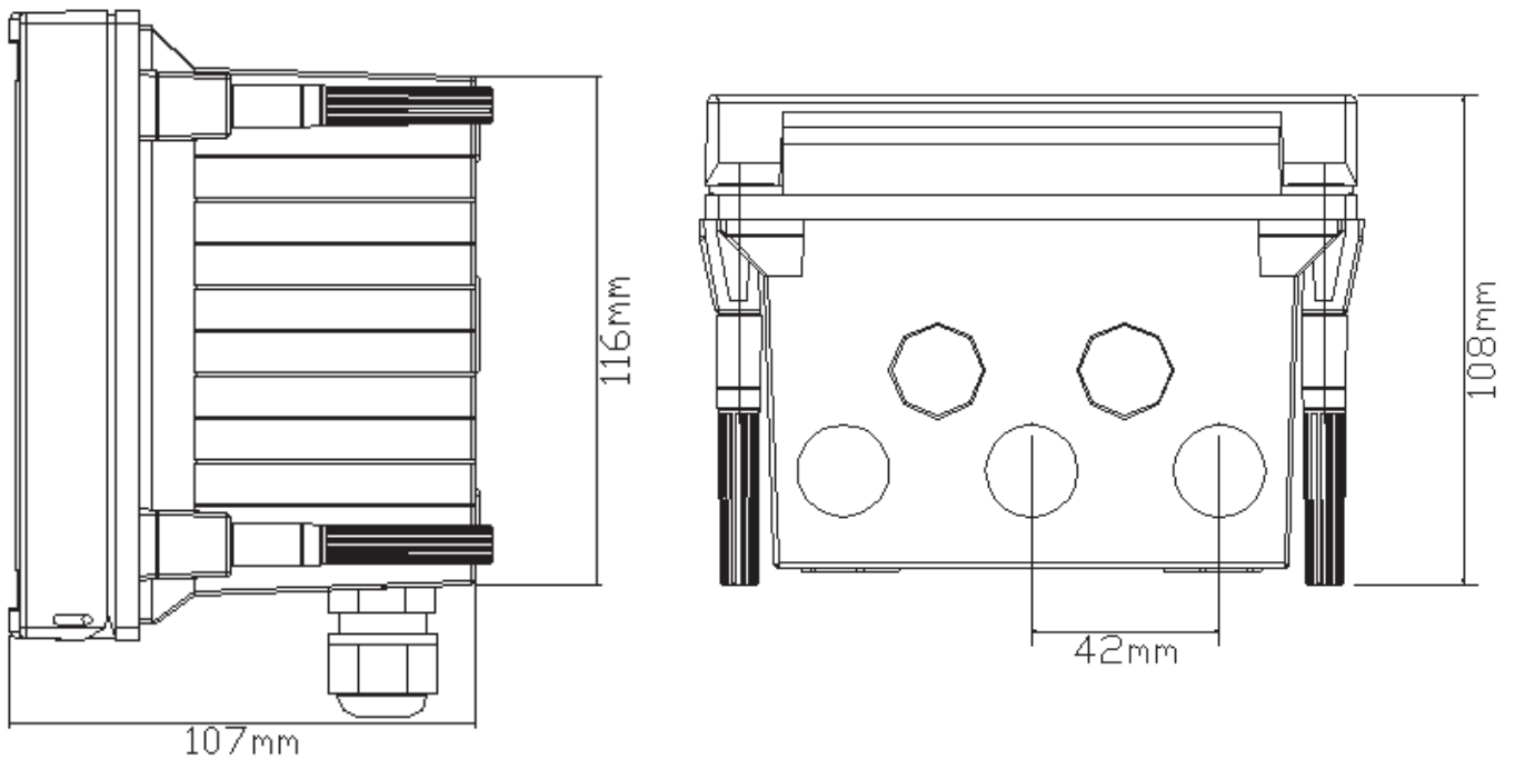
dimension
