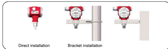
Direct installation
